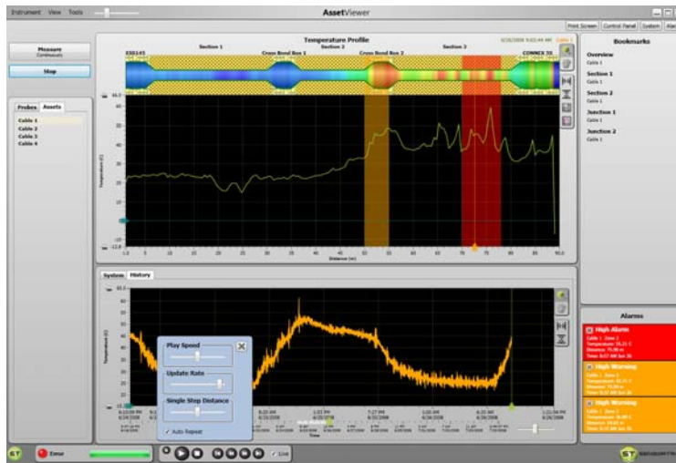
SensorTran AssetViewer™
